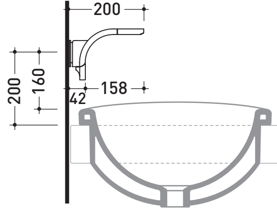
vista laterale / lateral view
